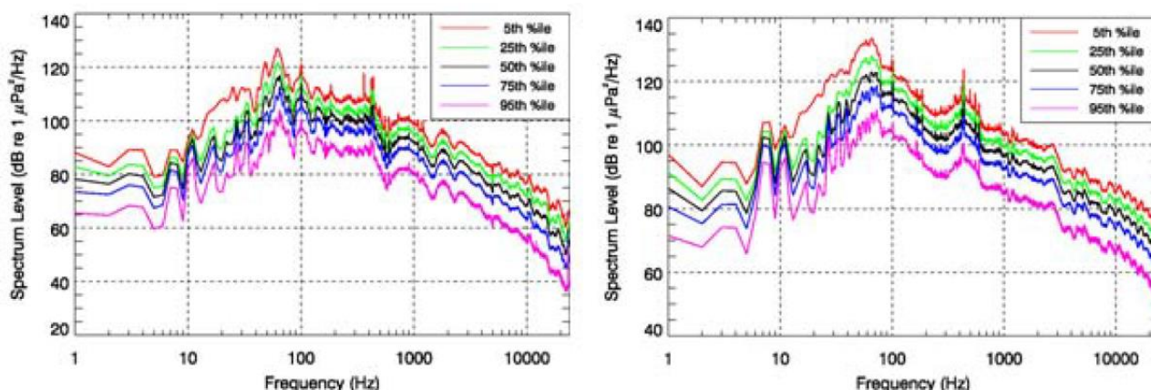
Figure 8.3: Frequency spectrum from measurement of underwater noise from survey vessel "Ocean Pioneer" in DP mode, measured at 207 m distance (left) and 74 m (right) (Reiser, Funk, Rodrigues, & Hannay, 2011).
