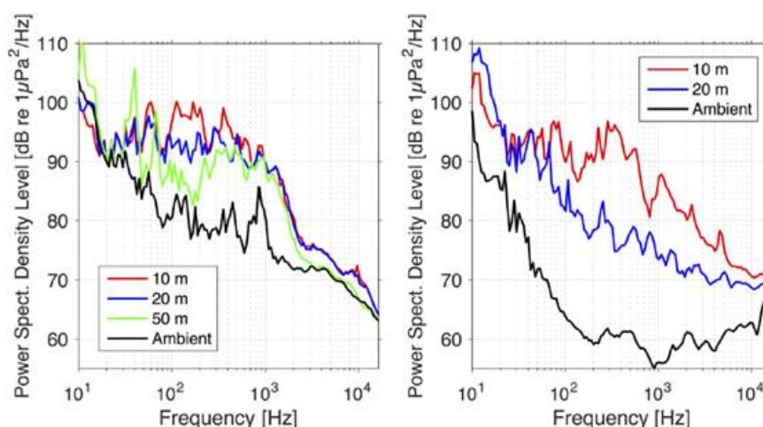
Figure 8.1: Frequency spectrum from underwater noise measurements of shallow water geotechnical drilling at Geraldton (left) and James Price Point (right) (Erbe & McPherson, 2017).
