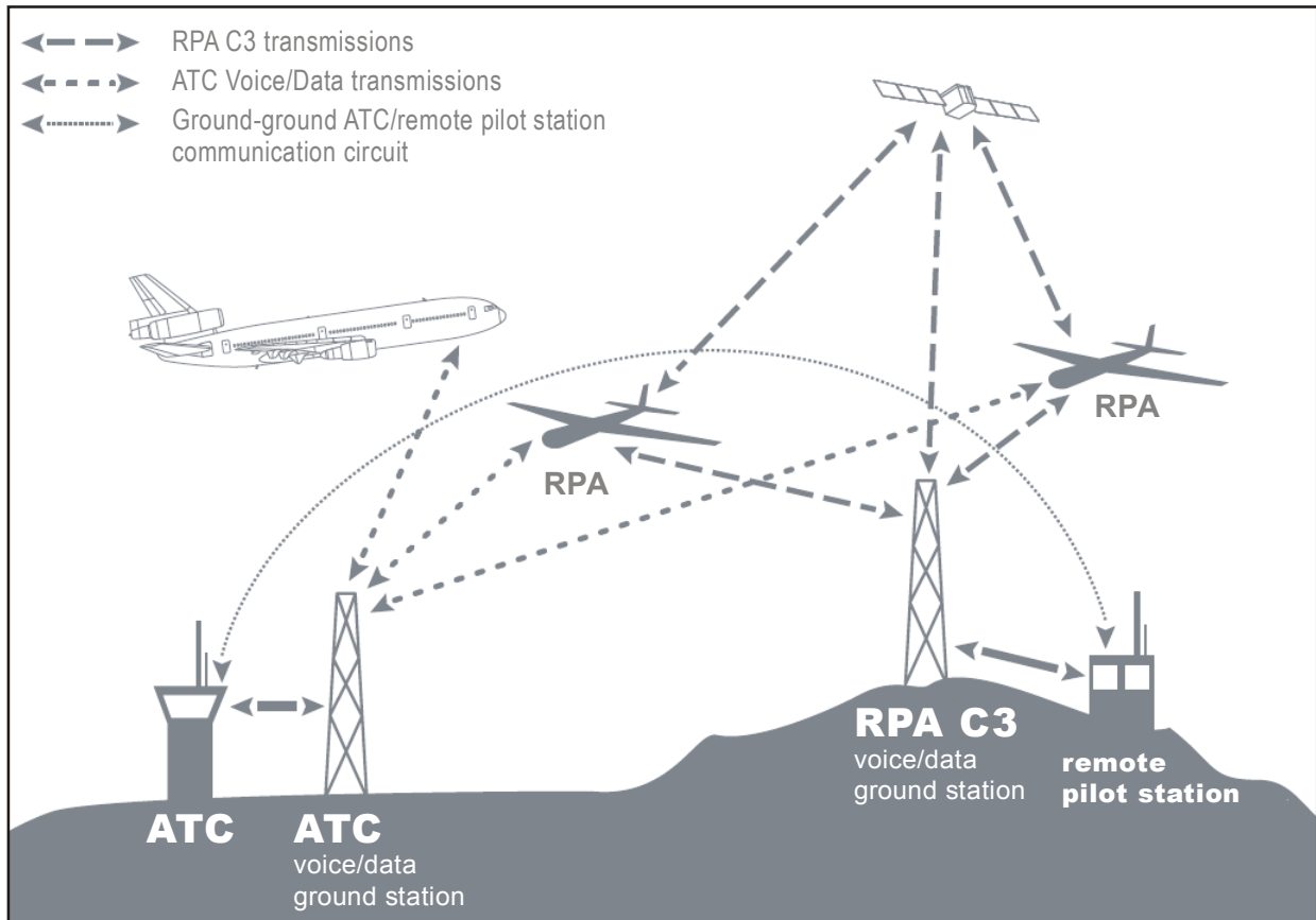
Figure 5-2. Communication links
